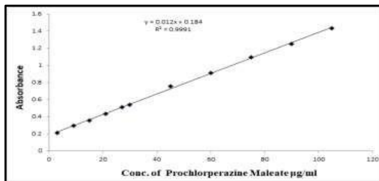
Figure 6. Calibration curve for determination Prochlorperazine Maleate
