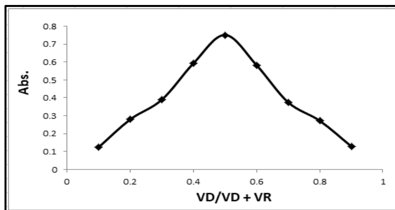
Figure 8. Continuous variations in output method (Job's method)
